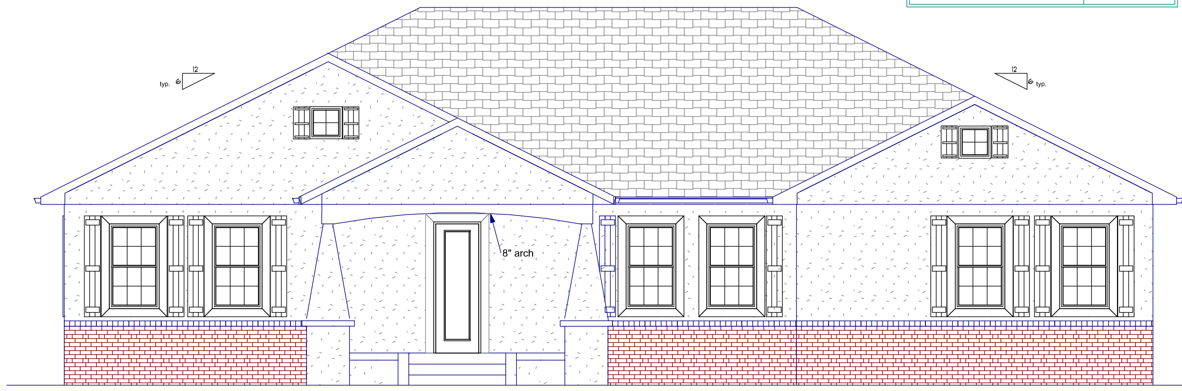
Front Elevation
