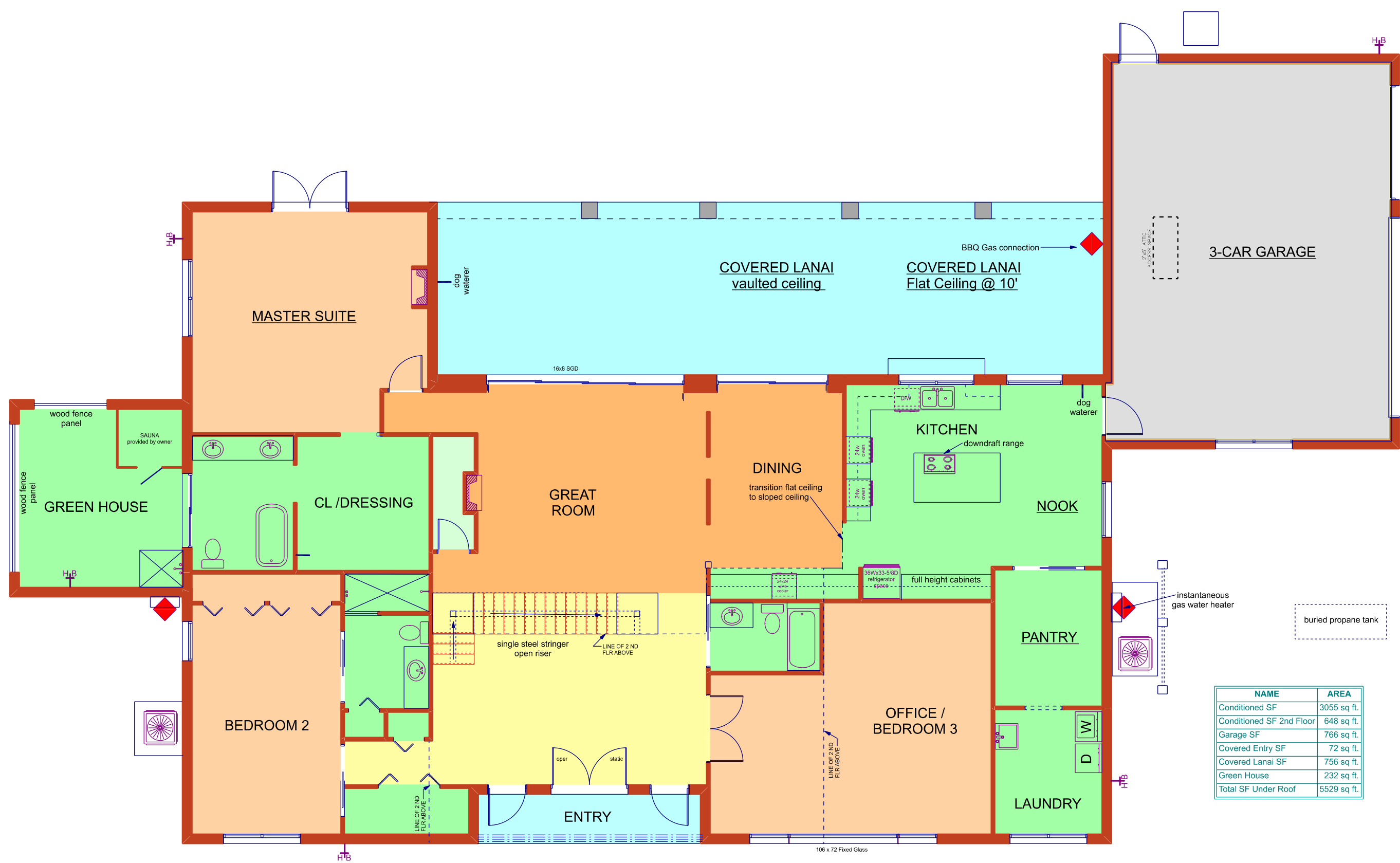
Calkins - First Floor Plan
