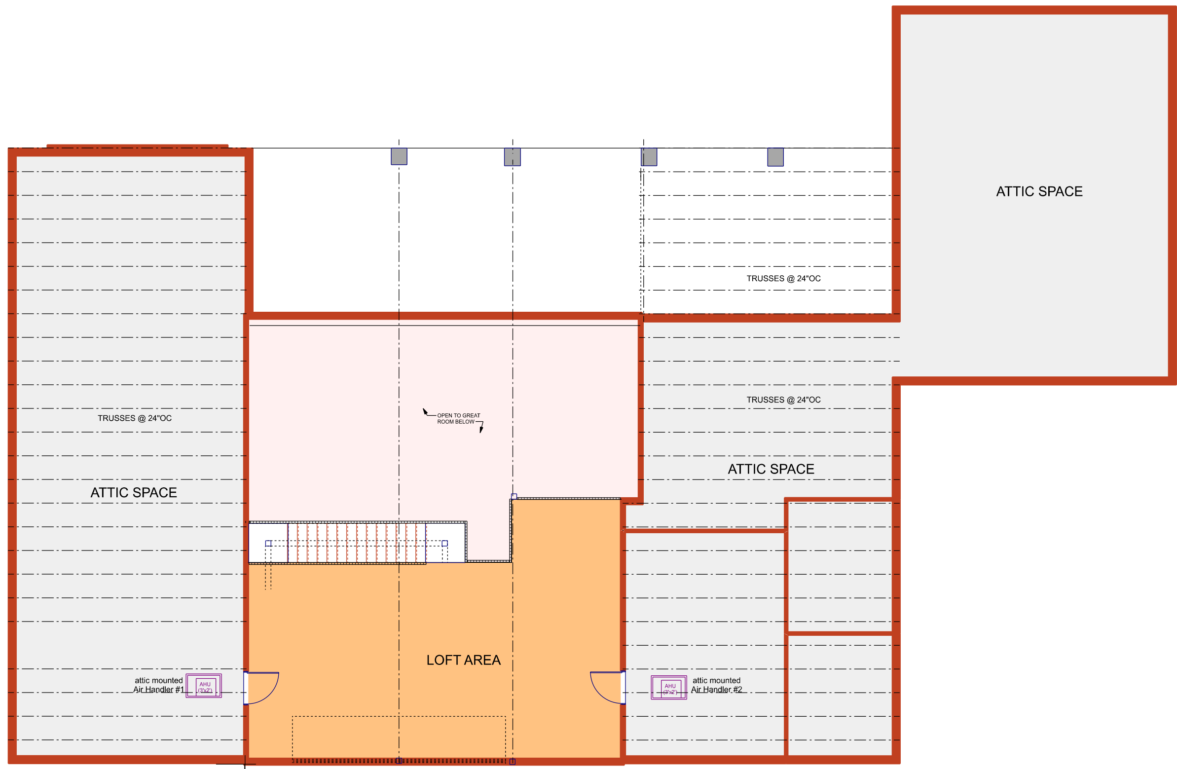
Calkins - Second Floor Plan
