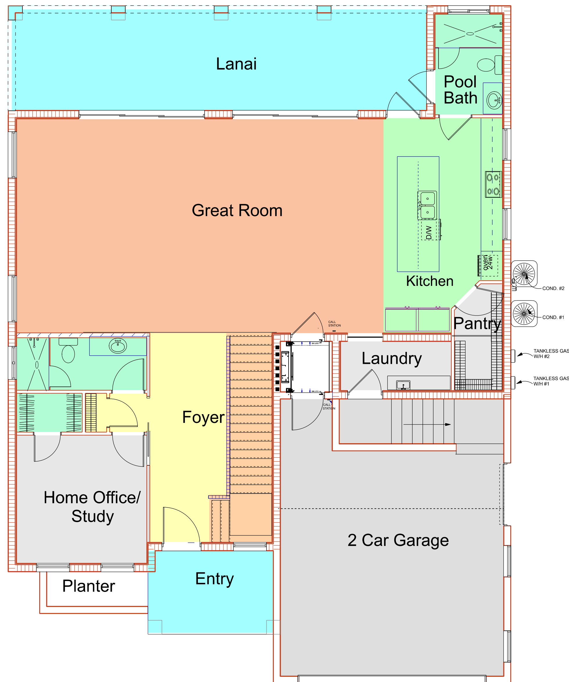
GRUMAN RESIDENCE FIRST FLOOR
